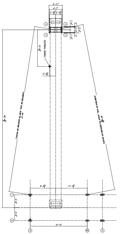
PLAN VIEW (SECTION A-A) * CONVEYOR CAN BE MOUNTED EITHER SIDE OF PLANT *
