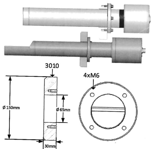
HPSE01/HPBX01
