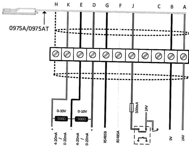
HP04/HPXT01/CA0022
